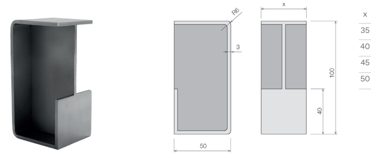
Tirador Didheya i-4250
